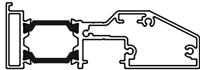
TWV-001 VENT FRAME GLAZE IN
