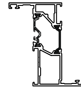
TWT-003 'Z' SECTION TRANSOM
