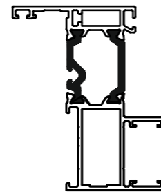
TWO-005 CURTAIN WALL INSERT OUTER OPEN OUT
