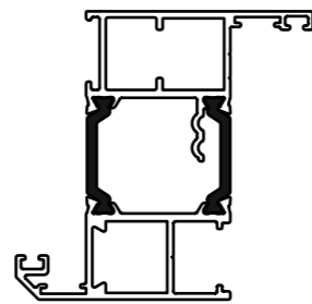
TWV-002 VENT FRAME GLAZE OUT
