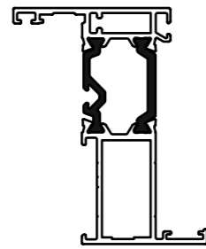
TWO-003 ODD LEG OUTER (GLAZE OUT)
