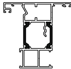
TWV-004 FLAT FACE VENT OPEN OUT GLAZE IN
