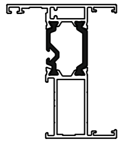
TWO-002 EQUAL LEG OUTER
