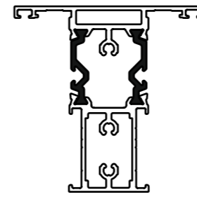
TWT-001 MULLION
