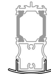
TWBP-004 150°-170° BAYPOLE COVER
