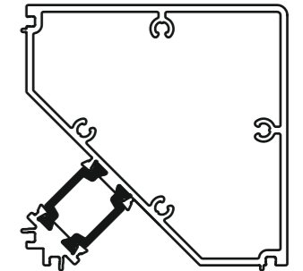
TWCP-001 SQUARE CORNER POST
