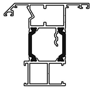
TWV-001 VENT FRAME GLAZE IN
