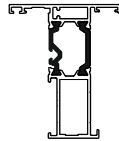
TWO-004 ODD LEG OUTER (GLAZE IN)
