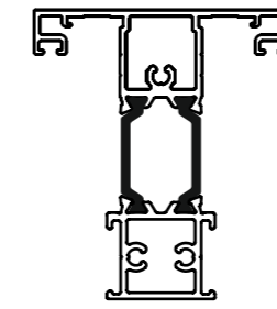
TWT-002 SLIM DUMMY TRANSOM/MULLION
