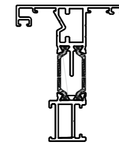
TWV-006 SLIM VENT OPEN OUT GLAZE IN
