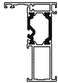
TWO-001 SLIM OUTER
