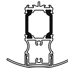
TWBP-003 130°-150° BAYPOLE COVER
