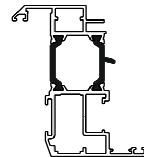
TWV-005 TILT/TURN VENT
