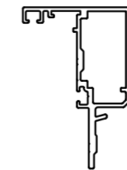
TWR-001 REBATE ADAPTOR
