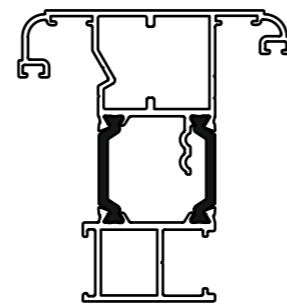
TWV-003 OVOLO VENT FRAME 2 (CRIMPED ONLY) GLAZE IN
