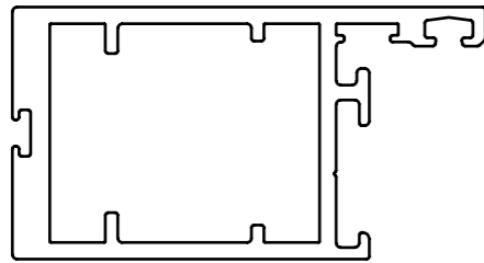
JID001 DOOR LEAF
