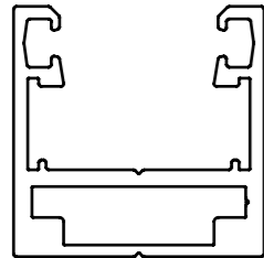
JID003 GLAZING CHANNEL
