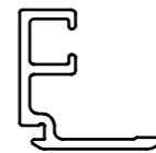
SWB-007 REBATED SASH BEAD INTERNAL
