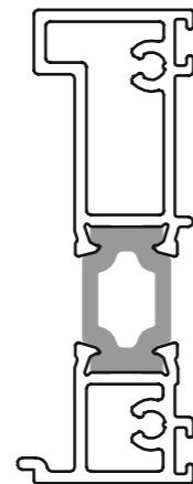
SDDC-001 BOTTOM RAIL CLOSER
