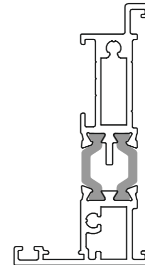
SDO-001 SLIM OUTER FRAME
