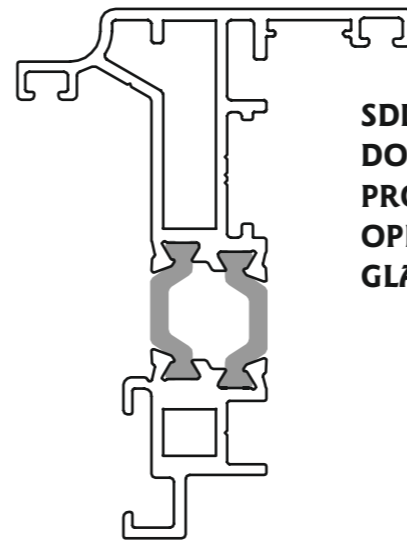
SDDC-001 BOTTOM RAIL CLOSER
