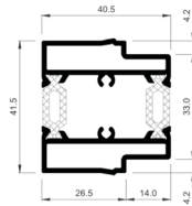
Sash joint profile
